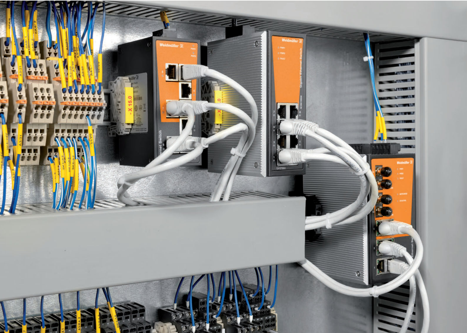
SAISM-4/8S-M12-4P D-COD
